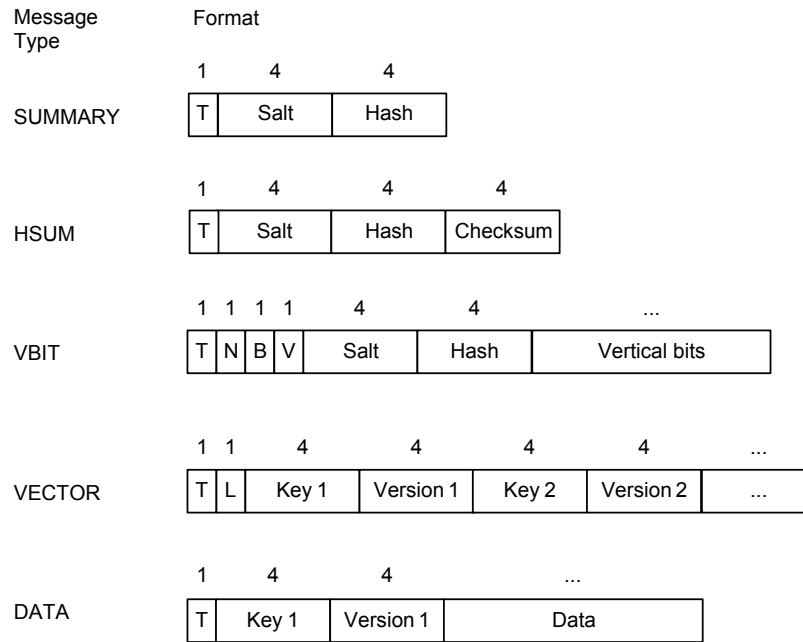
Figure 4.3: DHV message formats: (Source [1]: Used with permission from Springer Verlag)
