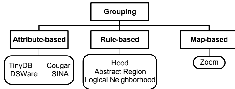
Figure 2.2: Grouping approaches
